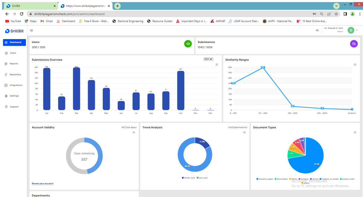
Figure 2: DrillBi Dashboard
