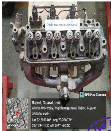
Cylinder Head with Cam Shaft Assembly
