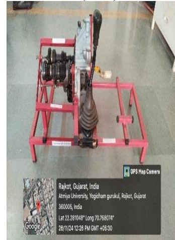
Transaxle Unit (FWD) Cut-Section
