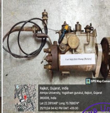
Fuel Injection Pump (Rotary)
