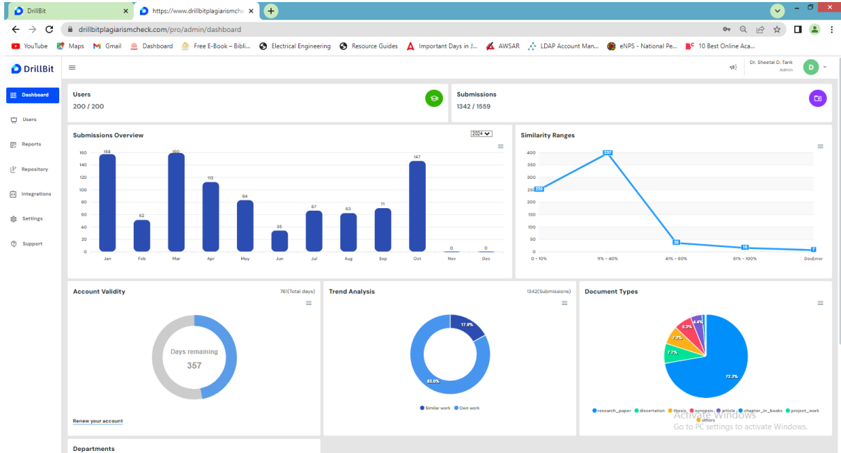
Figure 2: DrillBi Dashboard
