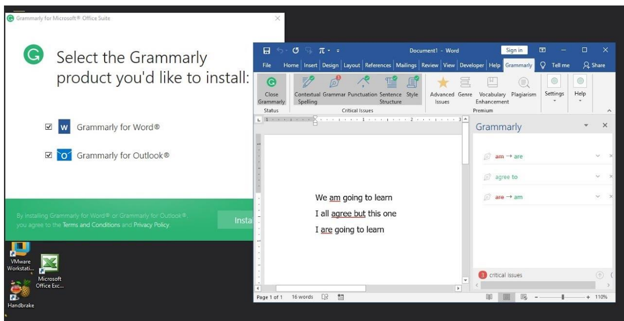
Figure 9: Grammarly
